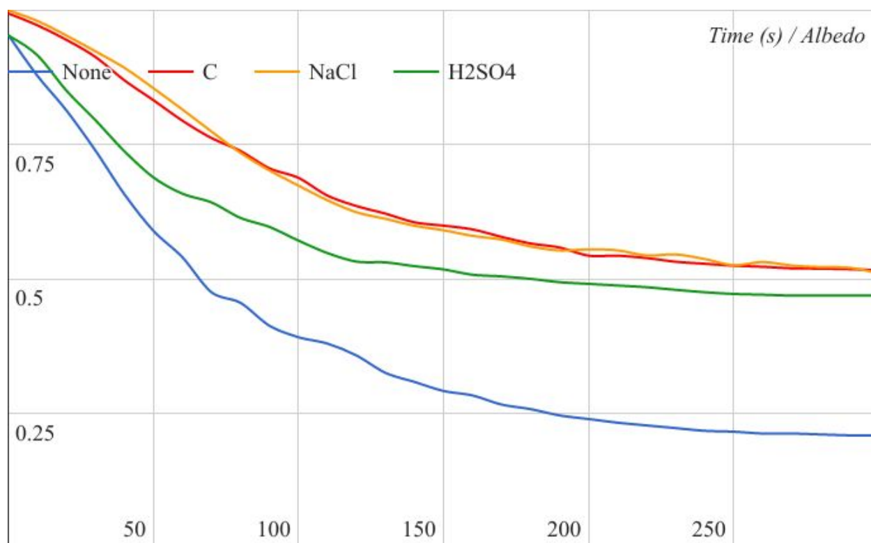
Chart 1. Average albedo vs. time for different aerosols
