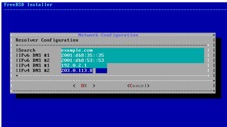
Figure 2.59. DNS Configuration
