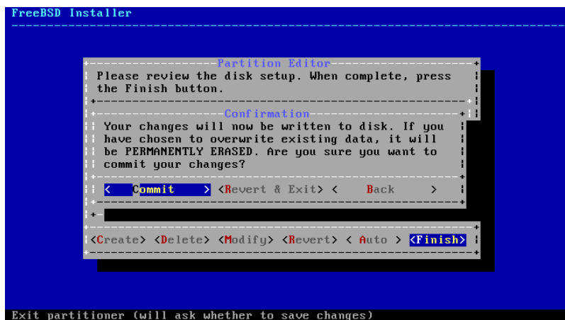
Figure 2.16. Final Confirmation
