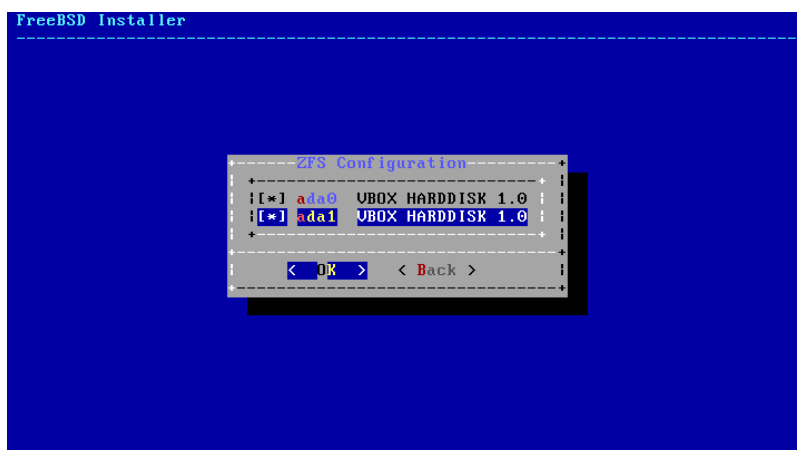
Figure 2.22. Disk Selection
