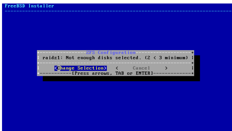
Figure 2.23. Invalid Selection
