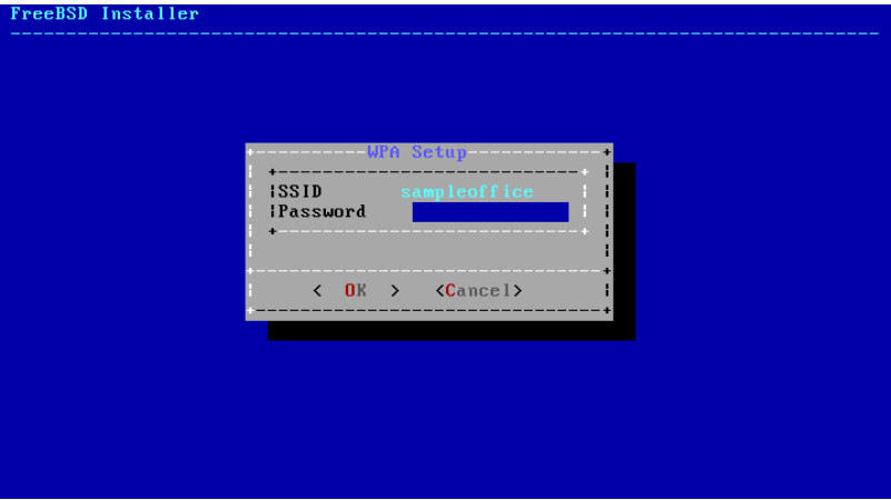
Figure 2.52. WPA2 Setup
