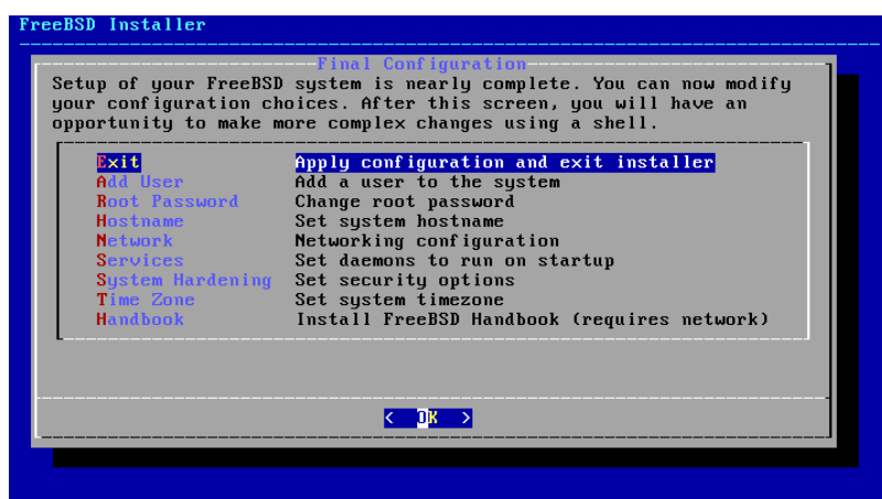
Figure 2.46. Final Configuration
