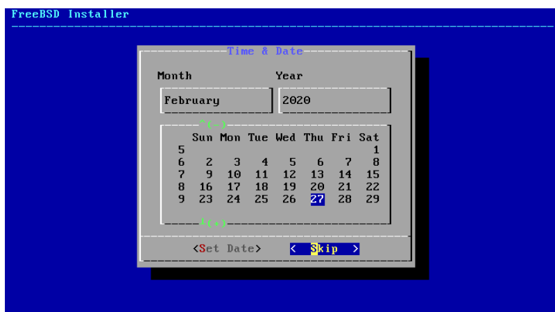
Figure 2.39. Select Date
