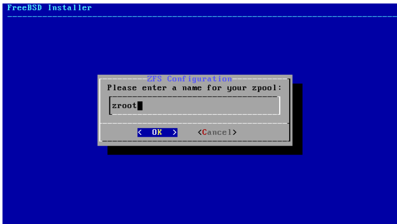
Figure 2.26. Pool Name
