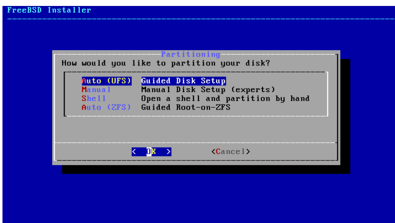
Figure 2.10. Partitioning Choices
