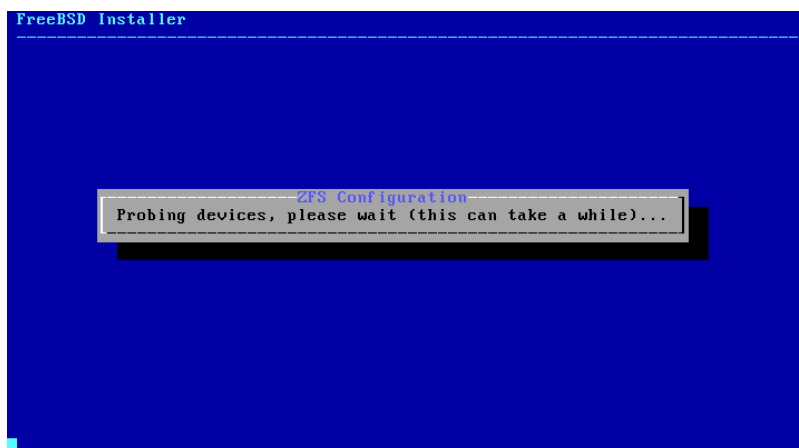
Figure 2.24. Rescan Devices
