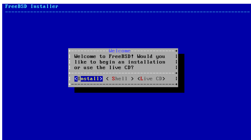
Figure 2.3. Welcome Menu
